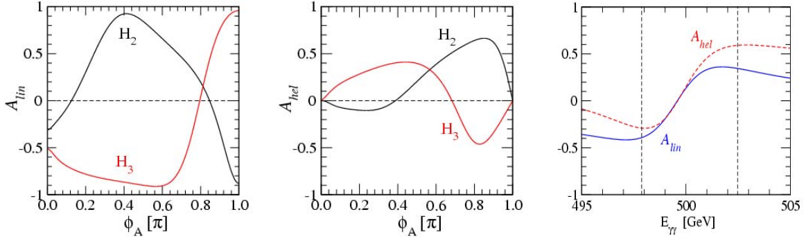
Figure 2: The \phi_A dependence of the CP-even and CP-odd correlators, \mathcal{A}_{lin} (left panel) and \mathcal{A}_{hel} (center panel), at the poles of H_2 and H_3 , respectively, and the \gamma\gamma energy dependence (right panel) of the correlators, \mathcal{A}_{lin,hel} , for \phi_A = 3\pi/4 in the production process \gamma\gamma \rightarrow H_i in the limit in which H/A mixing is the dominant CP-violating effect. The same parameter set as in Fig. 1 is employed. The vertical lines on the right panel mark positions of the two mass eigenvalues, M_{H_3} and M_{H_2} .
