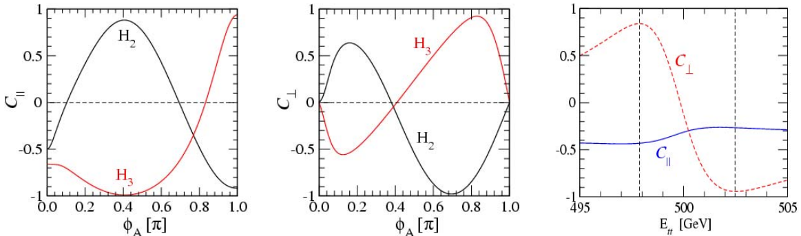
Figure 3: The \phi_A dependence of the CP-even and CP-odd correlators, \mathcal{C}_\parallel (left panel) and \mathcal{C}_\perp (center panel), at the pole of H_2 and H_3 and the invariant t\bar{t} energy dependence (right panel) of the correlators \mathcal{C}_{\parallel,\perp} for \phi_A = 3\pi/4 in the production-decay chain \gamma\gamma \rightarrow H_i \rightarrow t\bar{t} . [Same SUSY parameter set as in Fig.2.]
