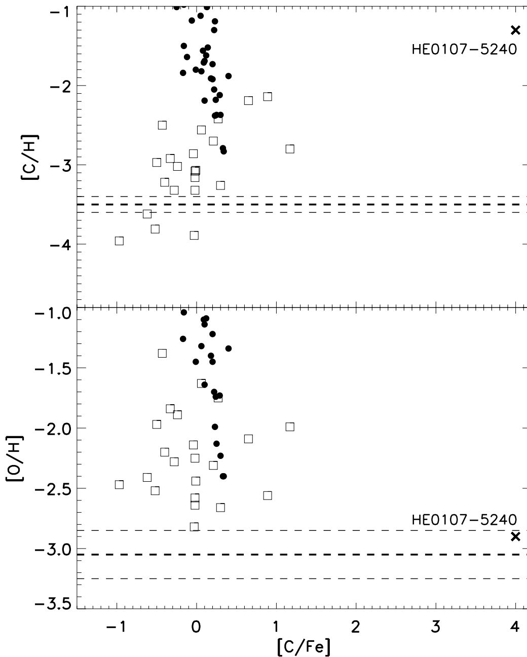
Figure 3: Observed abundances in low-metallicity Galactic halo stars. For both carbon ( upper panel ) and oxygen ( lower panel ), filled circles correspond to samples of dwarf and subgiant stars, and open squares to a sample of giant stars (see [7] for references). The dashed lines indicate the predicted critical carbon and oxygen abundances. Highlighted ( cross ) is the location of the extremely iron-poor giant star HE0107-5240. (Adapted from [7].)
