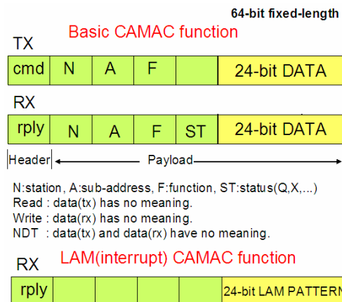
Figure 4: Frame format of CAMAC function
