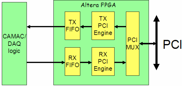
Figure 6: Architecture of PCI control
