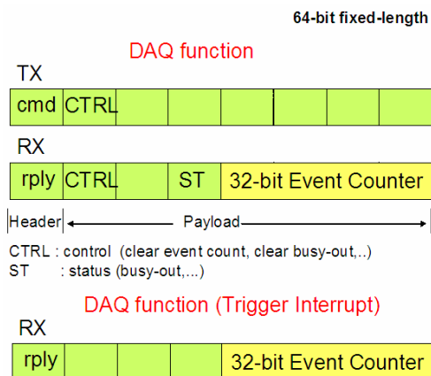
Figure 5: Frame format of DAQ function
