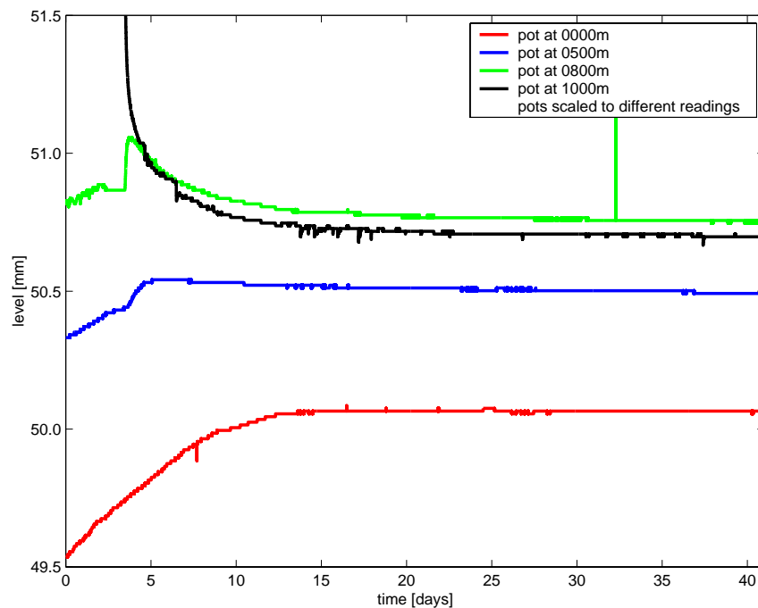
Fig. 9 leveling of water surface, tube diameter 20mm
