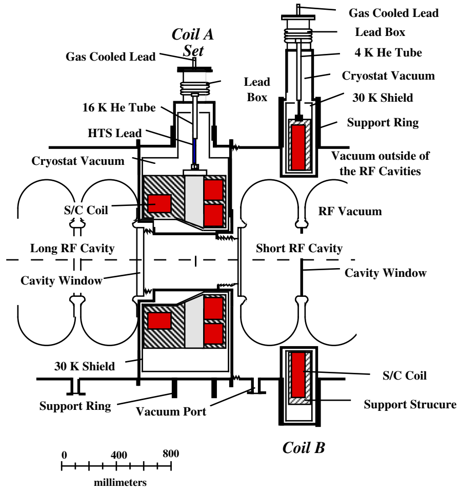
Figure 3: The matching section between the 2.75-m long and the 1.65-m long cooling cells. Half of a 2.75-m long magnet cell is on the left, and half of a 1.65-m long cell is on the right. There is no absorber within the A coils of this cell.
