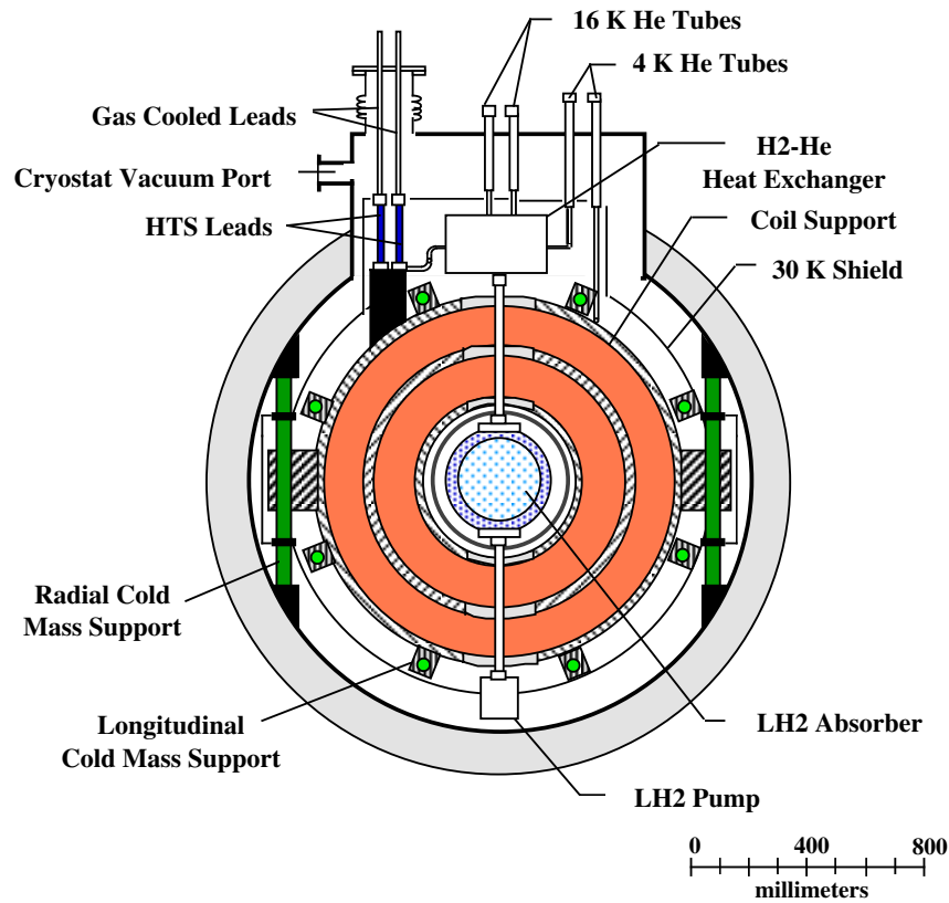
Figure 4: A Cross Section of the 1.65 m Cell A Magnet Perpendicular to the Beam. This figure shows the cold mass supports, the leads, cryogenic service ports, and the force carrying members that carry longitudinal magnetic forces up 1.3 MN.
