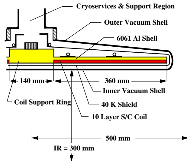
Figure 2: A cross section of the superconducting magnet for the induction cell downstream from the mini-cooler.
