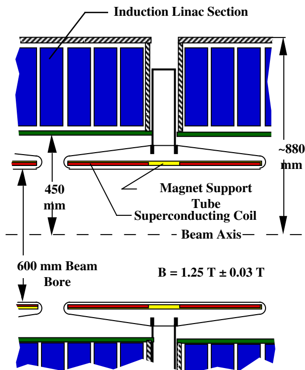
Figure 1: A cross section of the solenoid in an induction cell.
