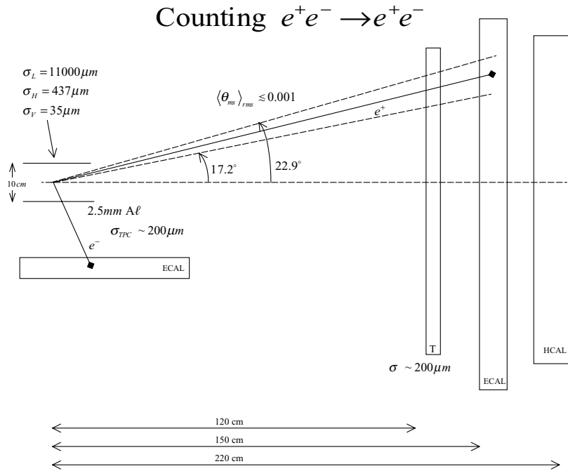
Figure 2: Geometry for counting Bhabha scatters.
