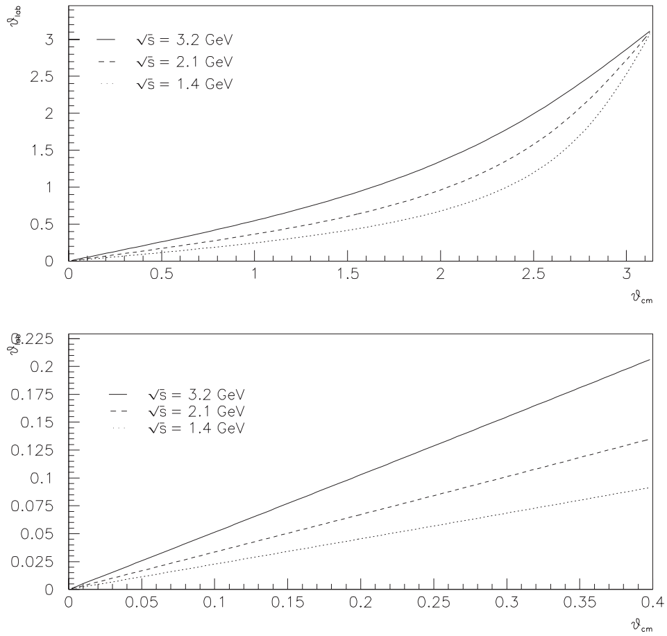
Figure 1: Bhabhas:laboratory v. center of mass angles.
