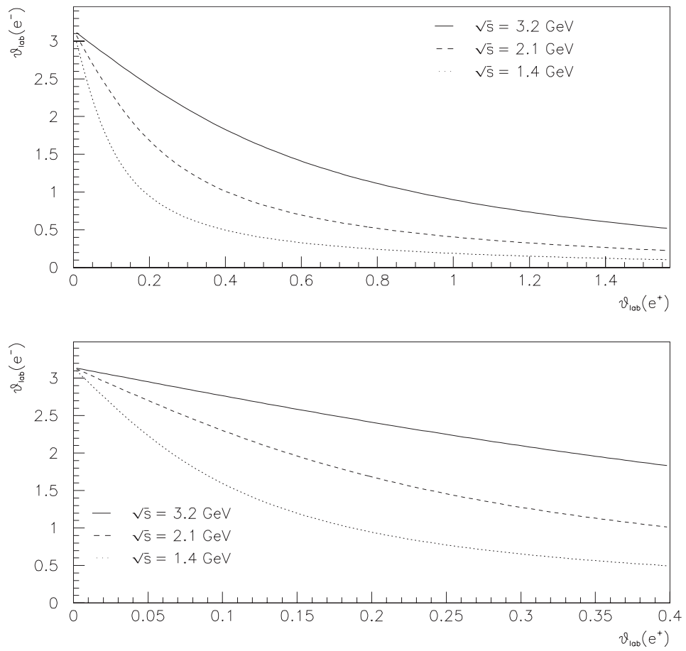
Figure 3: Bhabhas: electron v. positron laboratory angles.
