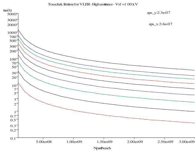
Figure 3: Touschek Lifetime at different beam energies.
