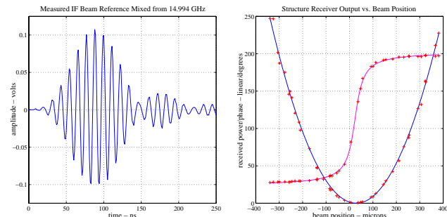
Fig. 9. IF waveform/results from structure alignment test. IF tone burst was digitized using a 1 GHz 8 bit VXI scope.
