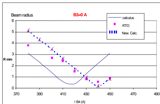
Figure 6 : Comparison of OTR measurements and calculus
