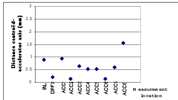
Figure 5 : Positon of the beam along the accelerator
