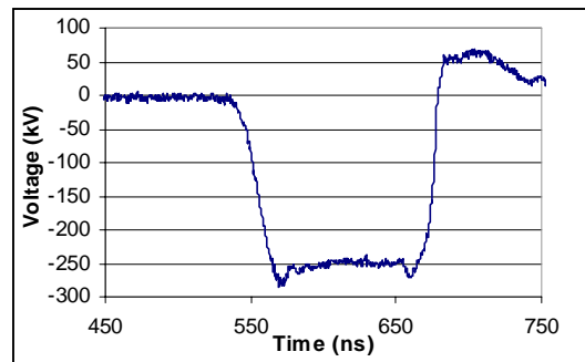
Figure 1 : Cell voltage signal synchronized with the electron beam
