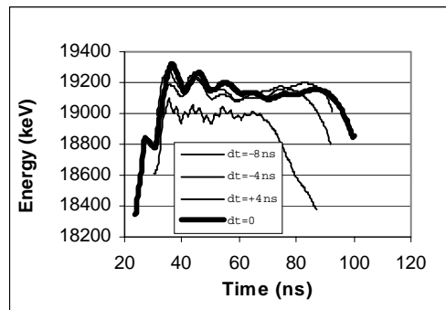
Figure 4 : Variation of duration of beam with synchronization of H.V. generators
