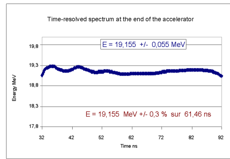
Figure 3 : Time resolved spectrum
