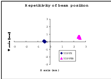
Figure 2 : beam position at the entrance and at the end of accelerator for 8 successive shots
