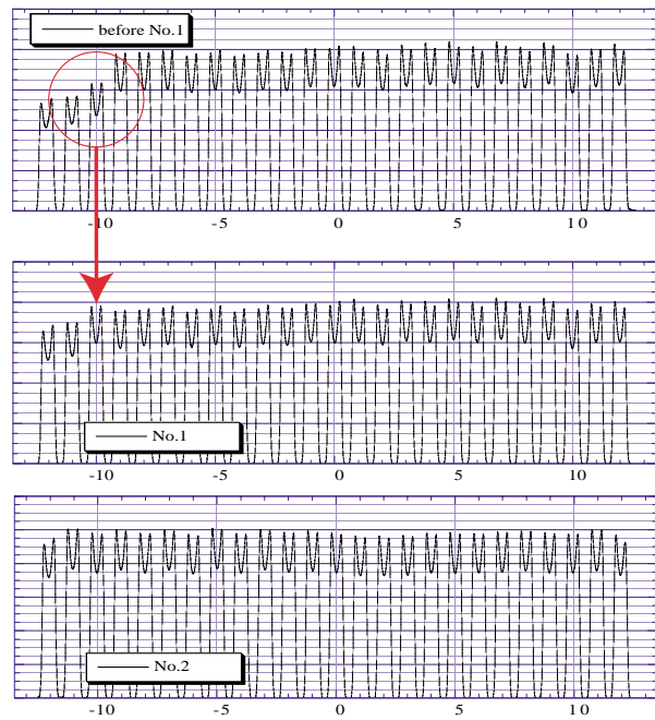
Figure 5: Correction of the electric field distribution and the final distributions of No.1 and No.2 accelerating tubes.
