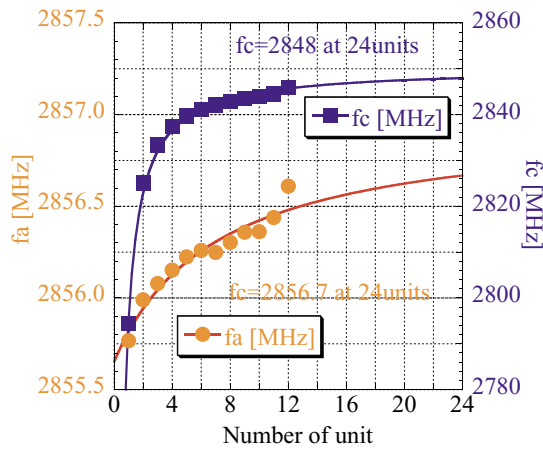
Figure 4: Unit number dependence on the accelerating and coupling mode frequencies.
