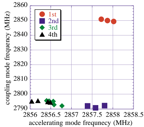
Figure 3: Single unit measurements of frequencies.
