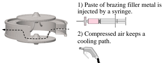
Figure 2: Repairing a vacuum leak by paste of brazing filler metal.
