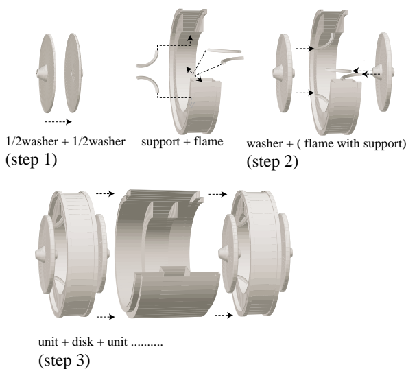
Figure 1: Fabrication steps of the biperiodic L-support DAW
