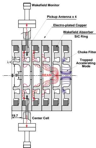
Figure 5: Shintake Choke-Mode Structure.
