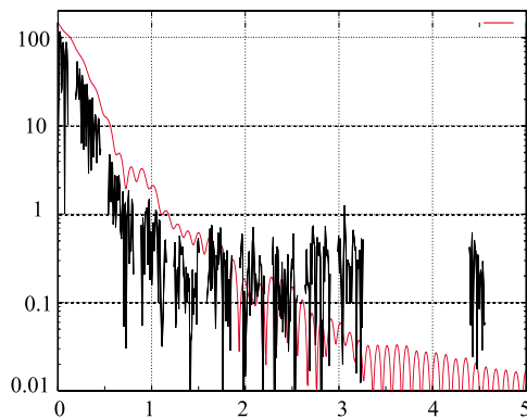
Figure 4: Plot of the measured and computed (smooth) transverse wakefields, V/(pC \cdot mm) vs. nanosec.
