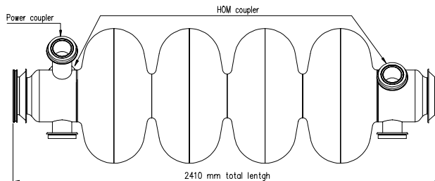
Figure 1: The LEP-2 accelerating cavity
