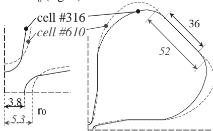
Fig. 1. RFQ cross-sections at two different locations.
