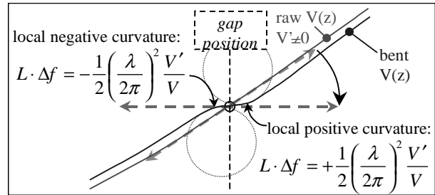
Fig. 4. Local bend of V(z) to get a horizontal tangent
