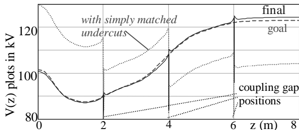
Fig. 7. Simulation of a segmented RFQ with a non-constant voltage law.
