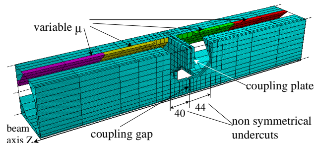
Fig. 5. Resonant coupling (as simulated in section 5).
