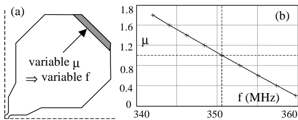
Fig. 6. Simulating \Delta f with a variable \mu zone.
