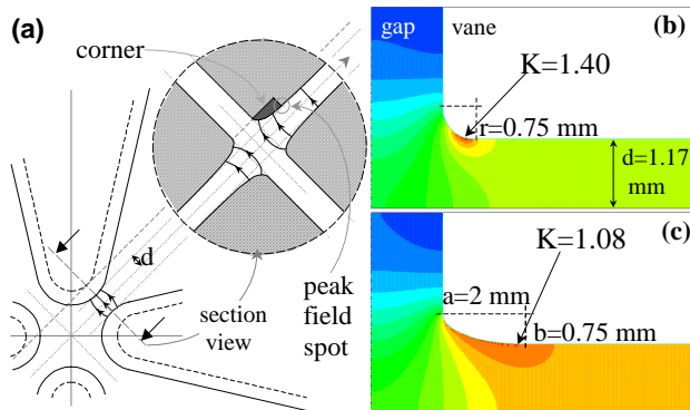
Fig. 8. Electrical field enhancement on vane ends: round corner (+40%), optimized elliptical corner (+8%).
