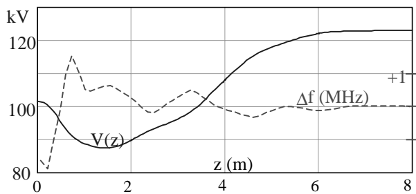
Fig. 3. Required voltage law and associated local \Delta f .
