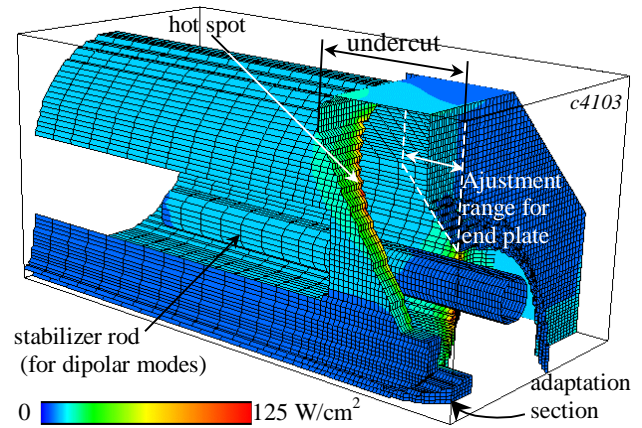
Fig. 2. Losses in IPHI RFQ input, computed with 'old' MAFIA: actually, the hot spot is still underestimated.
