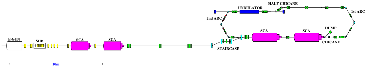
Figure 1: Schematic layout of the energy-recovery beam line.
