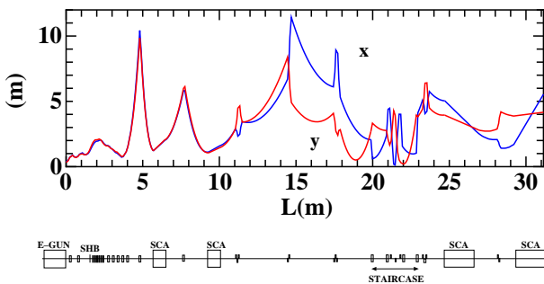
Figure 2: Horizontal and vertical beam envelope functions from the electric gun to the main-accelerator exit.
