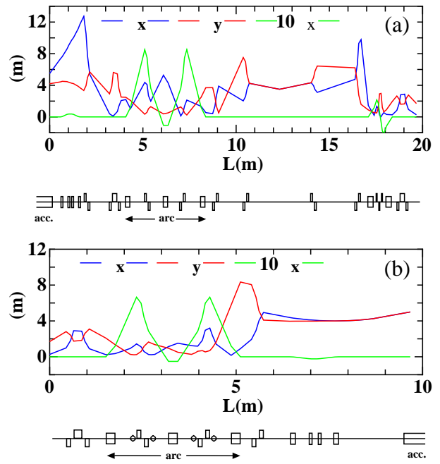
Figure 4: Horizontal and vertical beam envelope functions from the main-accelerator exit to the undulator entrance (a), and from the undulator exit to the re-injection point at the main-accelerator (b).
