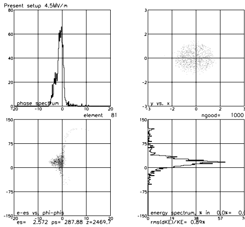
Figure 3: Various distributions of the longitudinal phase space at the entrance to the main cryomodule.
