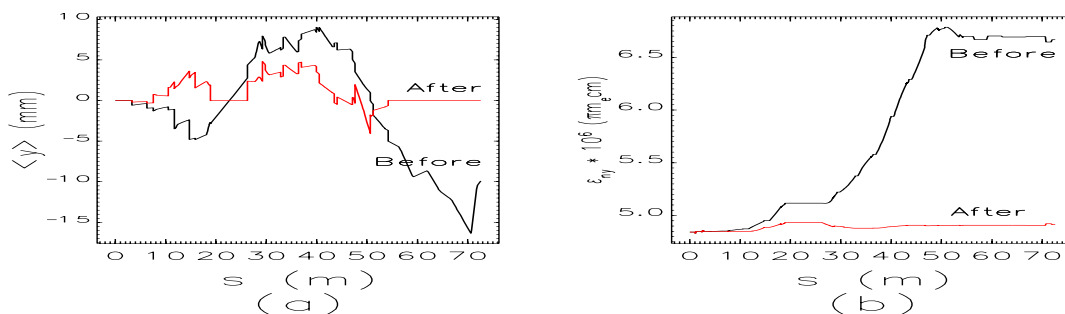
Figure 4: Trajectories (a) and emittances (b) before and after application of “ε-bumps.”
