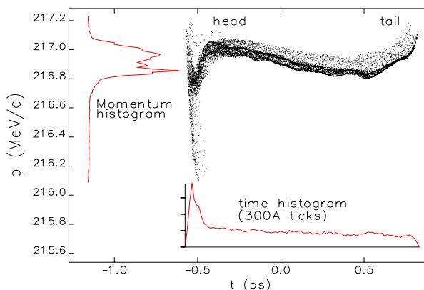
Figure 1: Typical longitudinal phase space (300-A case)
