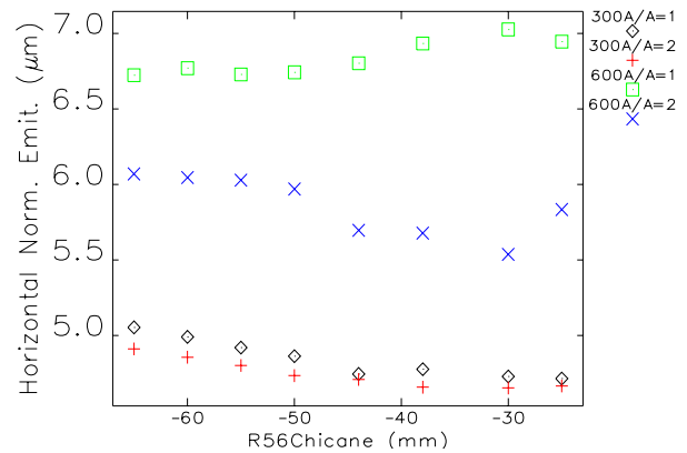
Figure 3: Horizontal normalized emittance vs. R_{56} .
