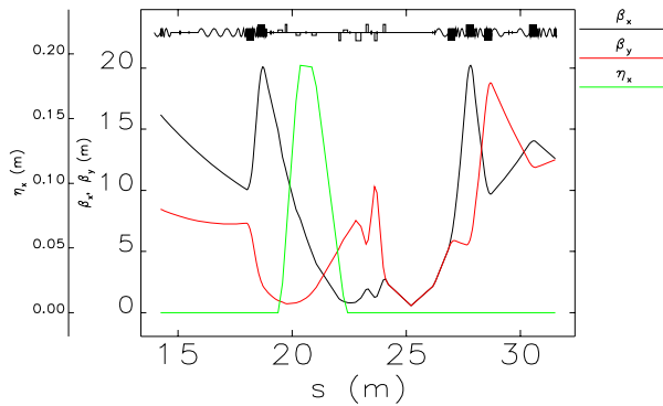
Figure 2: Typical Twiss parameters in the chicane region.
