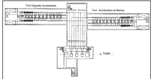
Figure 1: Basic layout of the IFMIF facility.
