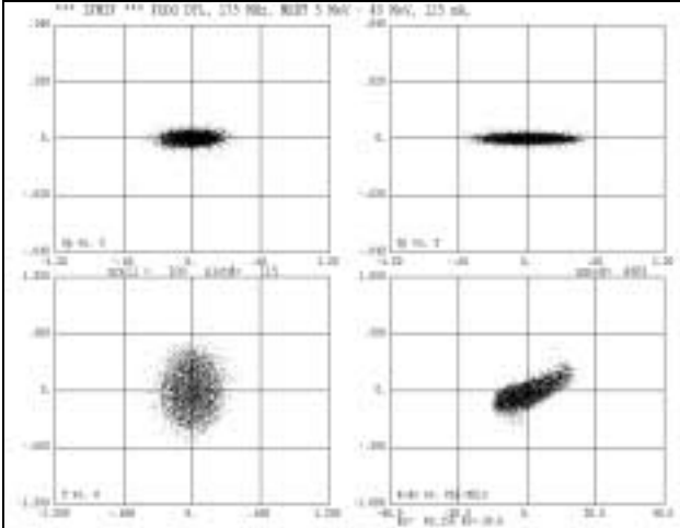
Figure 3: Output emittances of the 175 MHz DTL with a MEBT of 0.686 m between RFQ and DTL.
