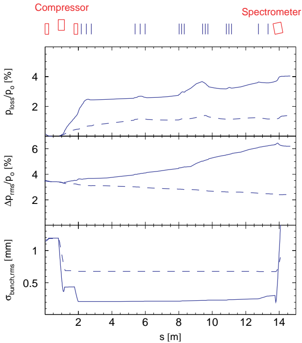
Figure 5: Evolution of the bunch length, the rms momentum spread and the momentum loss (from bottom to top) along the CTF II beam line as simulated with TraFiC 4 , for 10 nC. The results with two different setting of the chicane are shown, corresponding to R_{56} = 34 mm (solid line) and R_{56} = 15 mm (dashed line).
