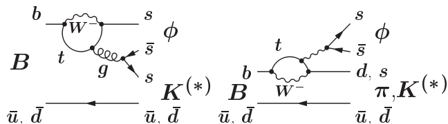
FIG. 1: Diagrams describing the decays B \rightarrow \phi K , \phi K^* , and \phi \pi : the dominant gluonic penguin (left), flavor singlet (right). In the latter, the s\bar{s} pair may be connected to the loop either through an electroweak boson ( \gamma , Z^0 ) or several gluons ( g ).
