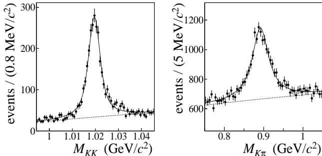
FIG. 2: The two-kaon invariant mass in the \phi signal region (left). Superimposed to the data is the fit to a relativistic P -wave Breit-Wigner for the \phi convoluted with a Gaussian on top of a polynomial background. The mass resolution is 1.1 \text{ MeV}/c^2 . The plot to the right shows a Breit-Wigner fit to the K^0\pi^+ invariant mass in the K^{*+} signal region. Both fits use Breit-Wigner parameters from Ref. [8].
