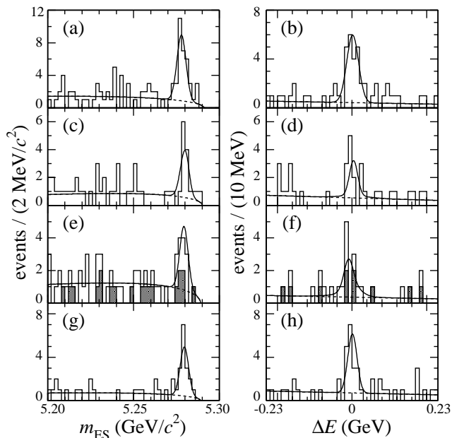
FIG. 3: Projections onto the variables m_{ES} (left) and \Delta E (right). The histograms show data for (a,b) B^+ \rightarrow \phi K^+ ; (c,d) B^0 \rightarrow \phi K^0 ; (e,f) B^+ \rightarrow \phi K^{*+} ; (g,h) B^0 \rightarrow \phi K^{*0} after a requirement on the signal probability \mathcal{P}_{\text{sig}}/\Sigma\mathcal{P}_i with the PDF for m_{ES} or \Delta E excluded. In (e,f) the histogram is the sum of the two \phi K^{*+} channels while the shaded area is K^{*+} \rightarrow K^0\pi^+ alone. The solid (dashed) line shows the signal-plus-background (background only) PDF projection.
