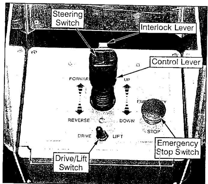
Figure 2: Controller
