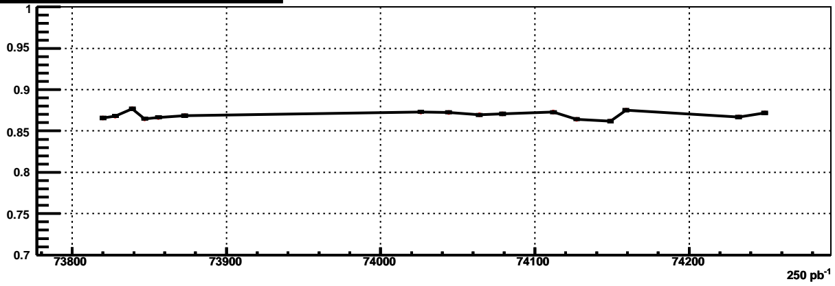
Lum Ratio Mupair over mupair(BC) 250 pb -1
