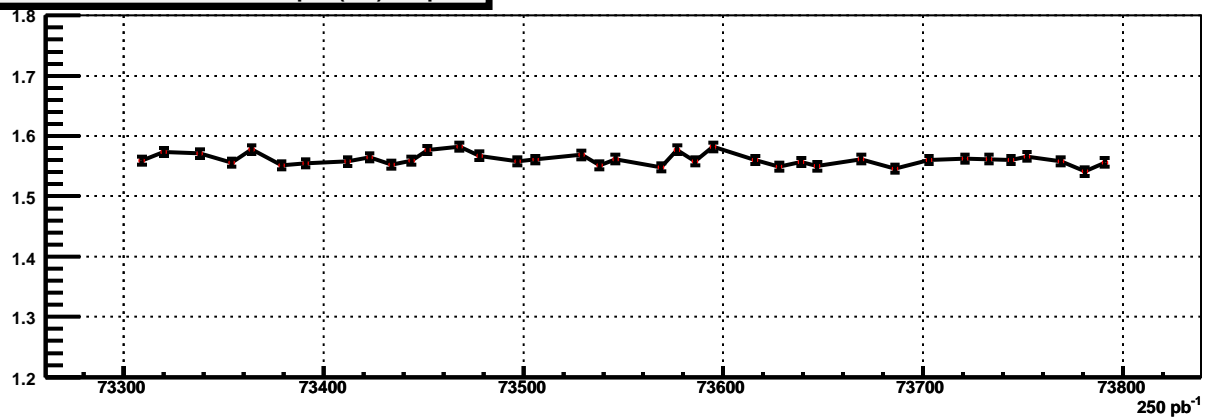
Lum Ratio GammaGamma over mupair(BC)250 pb -1
